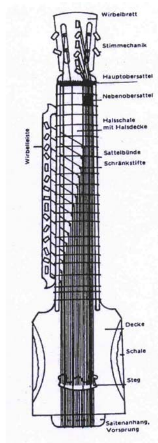
Abb. 9: Surbahar
